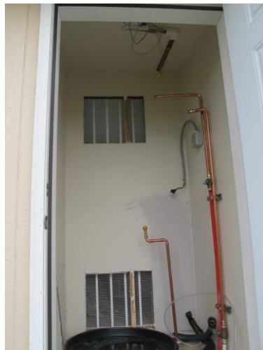
Figure 3.4. Transfer Grille and Thermostat Locations. Left: transfer grilles (25-inch \times 20-inch) installed between water heater closet and adjacent master bedroom closet. Right: location of grilles on wall 1) between water heater closet and master bedroom closet and 2) between master bedroom closet and hallway to provide sufficient free airflow to the water heater closet
