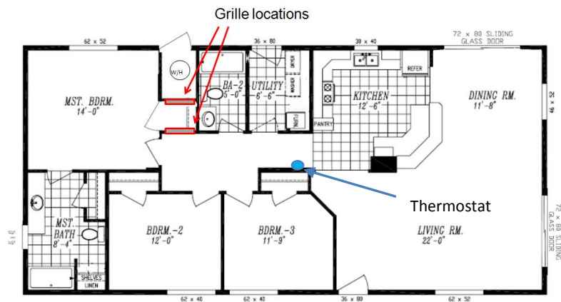
Figure 3.4. Transfer Grille and Thermostat Locations. Left: transfer grilles (25-inch \times 20-inch) installed between water heater closet and adjacent master bedroom closet. Right: location of grilles on wall 1) between water heater closet and master bedroom closet and 2) between master bedroom closet and hallway to provide sufficient free airflow to the water heater closet
