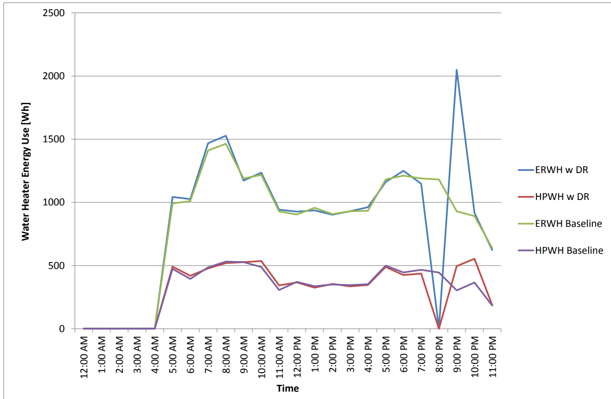
Figure 4.18. Evening INC Balancing Event Hourly Average Water Heater Energy Use Profile for the HPWH and ERWH with and without DR Signals (W·h)
