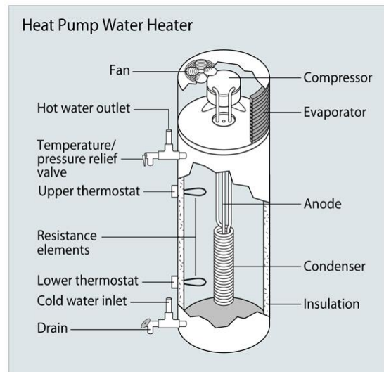
Figure 3.2. Diagram of Key Components in a Unitary HPWH. Source: U.S. DOE; energysavers.gov.
