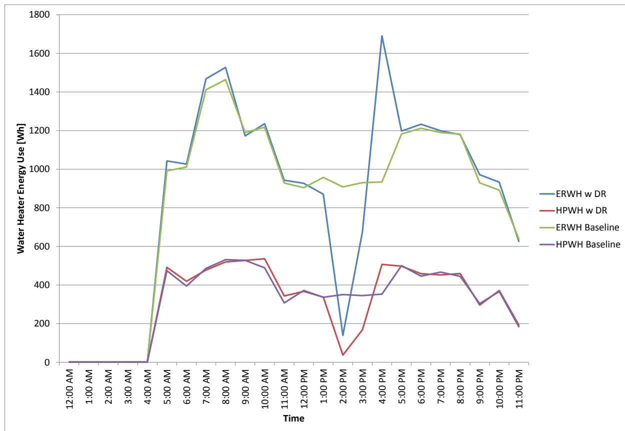
Figure 4.16. Afternoon INC Balancing Event Hourly Average Water Heater Energy Use Profile for the HPWH and ERWH with and without DR Signals (W·h)
