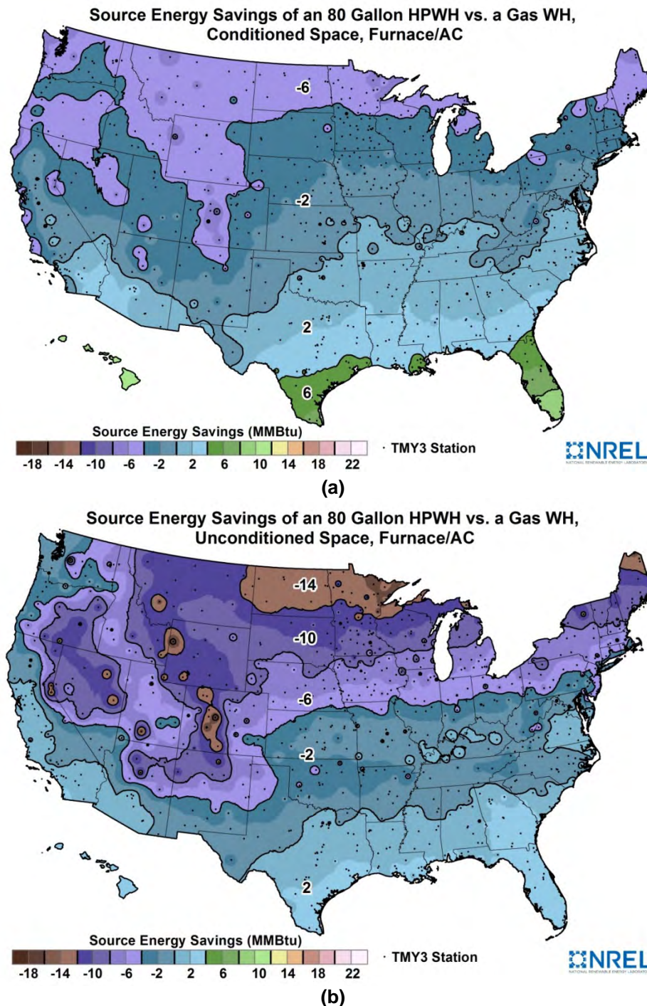
Figure 23. Source energy savings of an 80-gal HPWH relative to a gas WH for a home with a furnace/AC when the WH is in (a) conditioned and (b) unconditioned space
