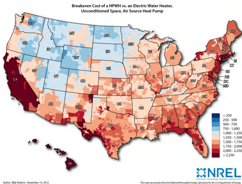
Figure 12. Breakeven cost of a 50-gal HPWH relative to an electric WH for a home with an ASHP when the WH is in (a) conditioned and (b) unconditioned space
