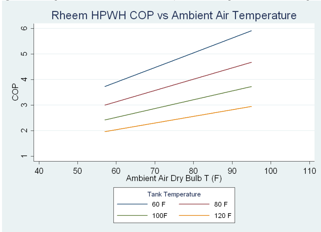
Figure 4. The plots are fits to measured data. (COP-95d test point excluded from plot).
