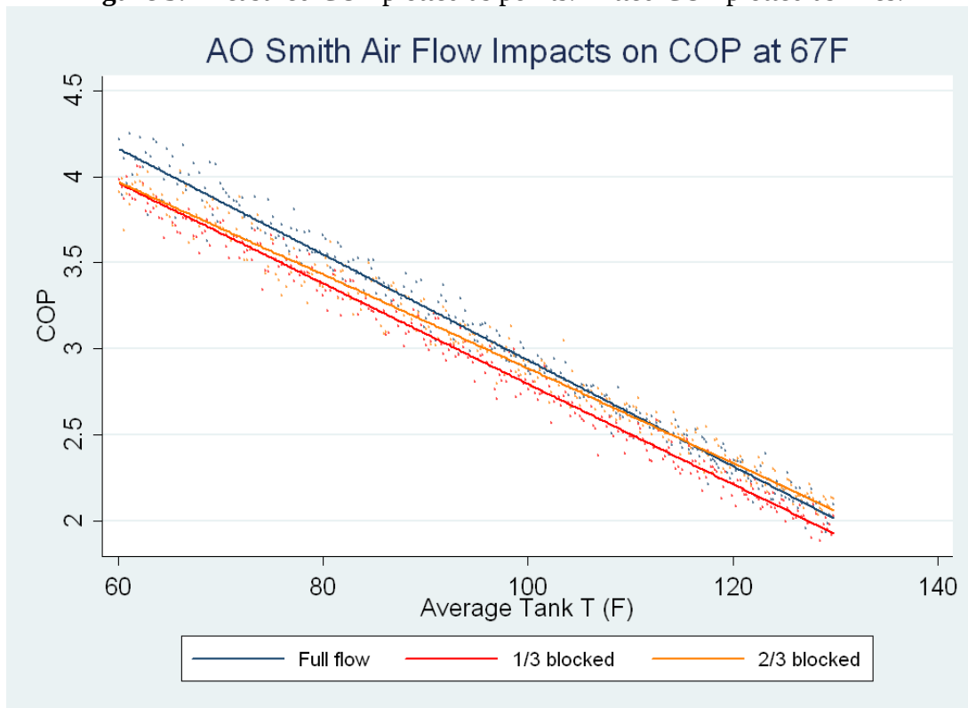
Figure 5. Measured COP plotted as points. Fitted COP plotted as lines.
