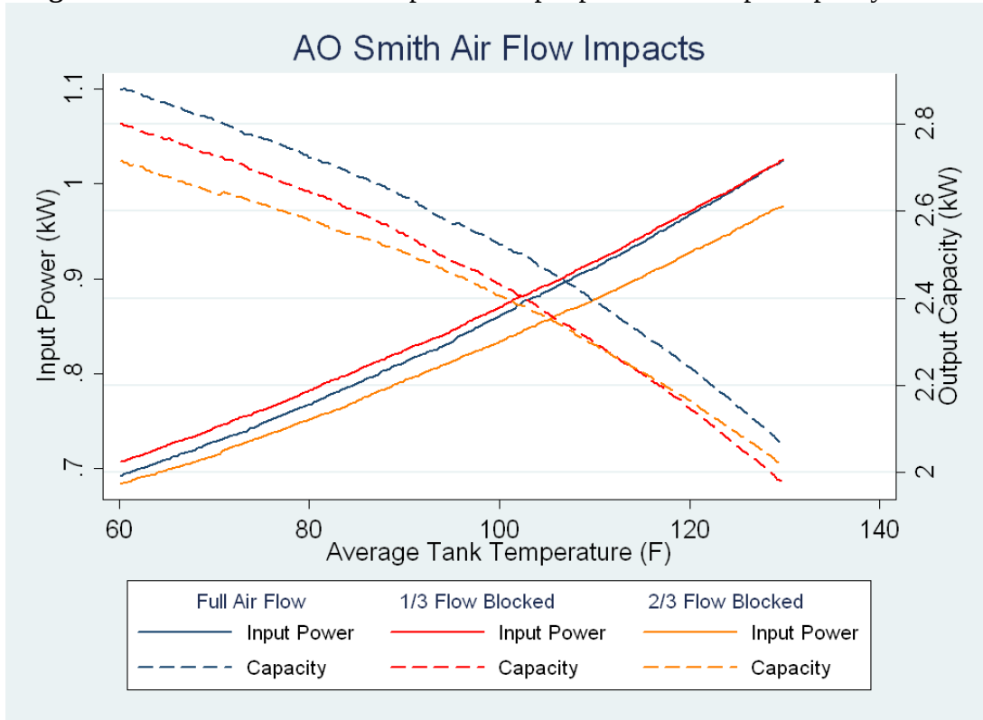
Figure 6. Air flow restriction impacts on input power and output capacity at 67F.
