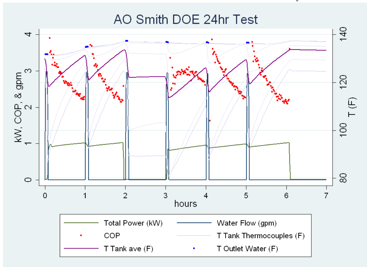
Figure 2a. DOE 24hr Simulated Use Test.
