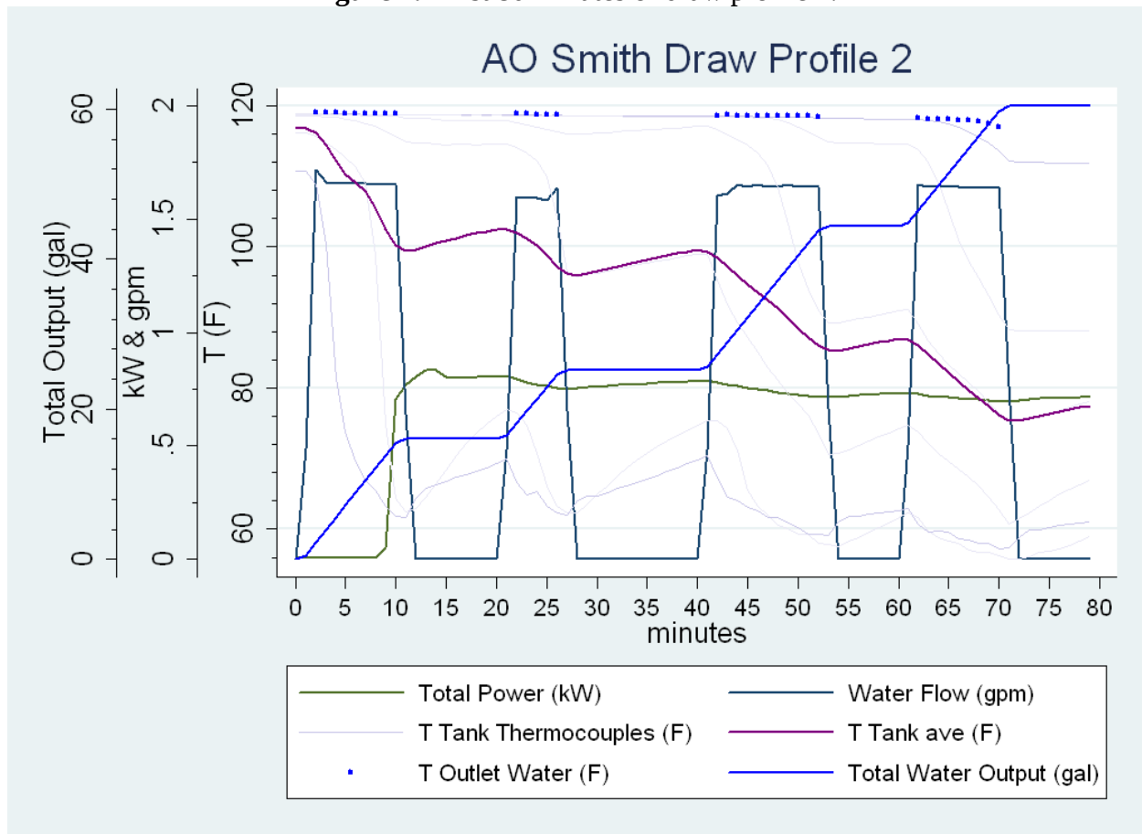
Figure 7. First 80 minutes of draw profile 2.
