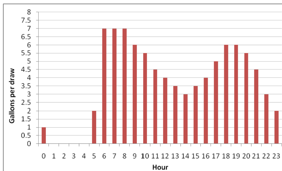
Figure 4. Draw profile (1).
