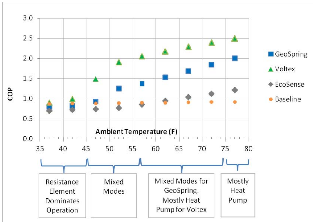
Figure 30. COP Map
