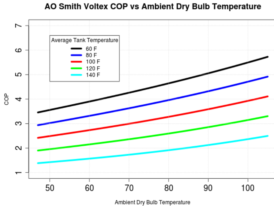
Figure 16. Voltex COP vs Ambient Temperature
