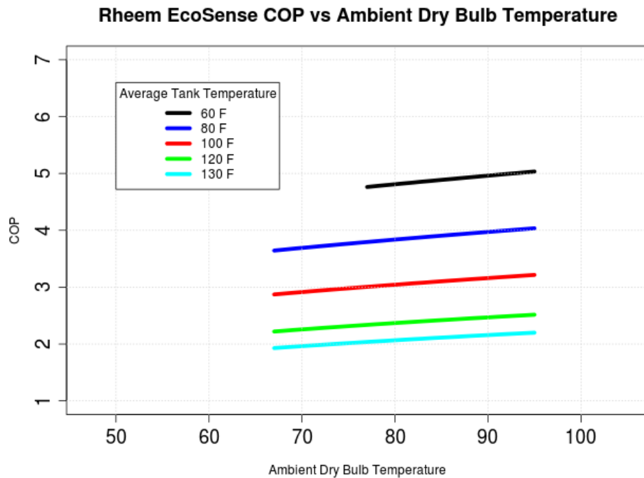
Figure 20. EcoSense COP vs Ambient Temperature
